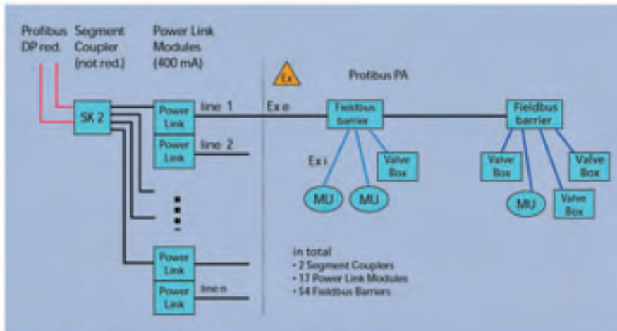
Figure 1: Topology of the fieldbus reference solution
